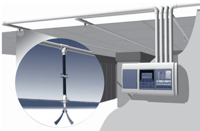
Figure 2. Xtralis VESDA Pipe Network
